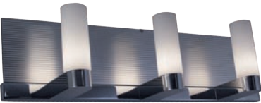
M1803W / reflex 3 x G9-40W L 20" (508 mm) D/P 4¼" (108 mm) H 5" (127 mm) Chrome - Mirror, Textured aluminium Chrome - Miroir, Aluminium texturé
