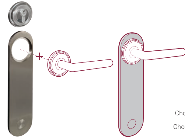
KPE300SS Set : Back plate + deadbolt Kit : Plaque + pêne dormant
